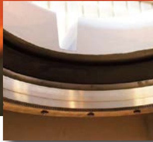
Graphite Ring Installed in Billet Casting Mold
